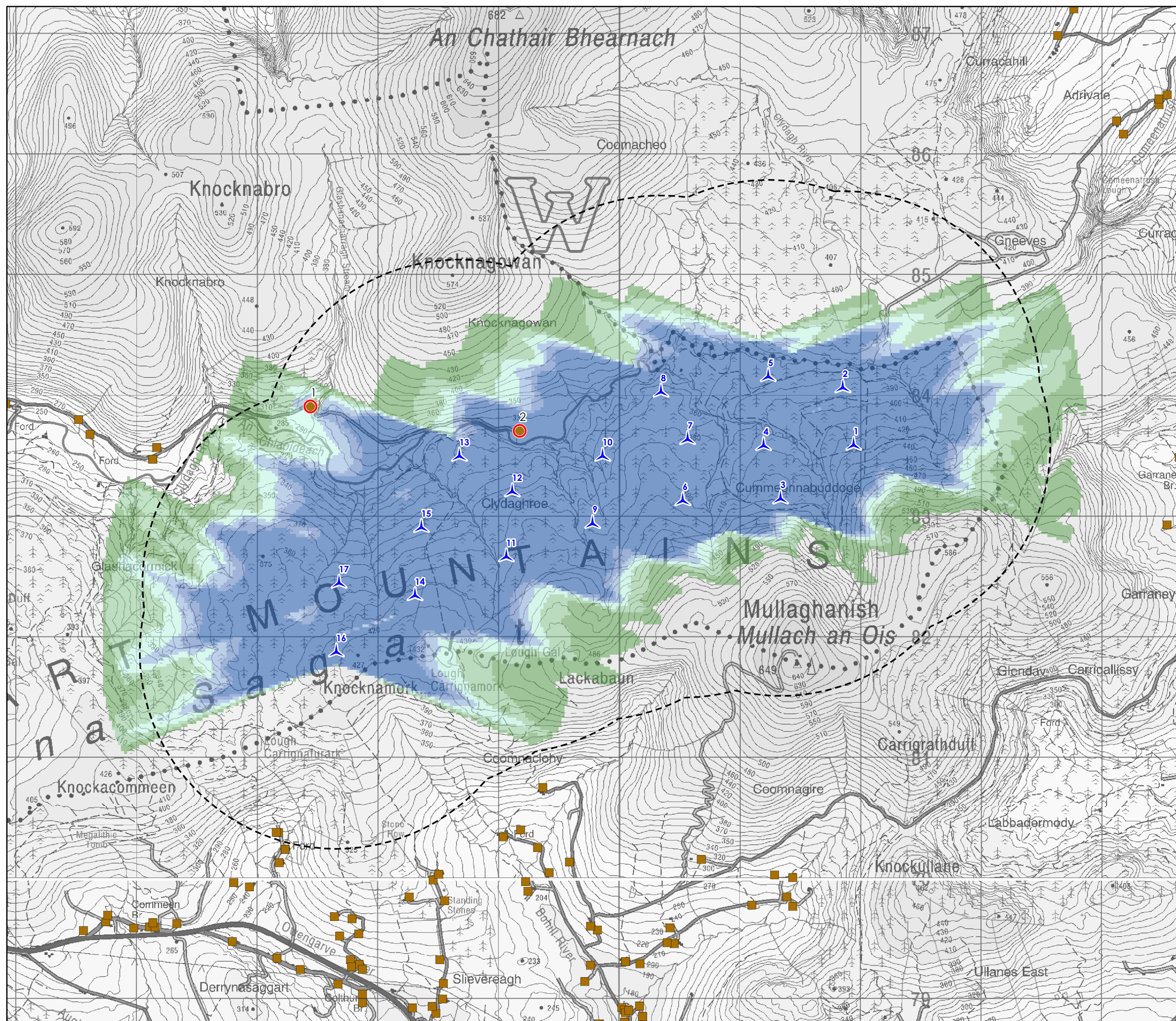
Figure 15-1a Shadow Flicker Assessment - Maximum Rotor Diameter
